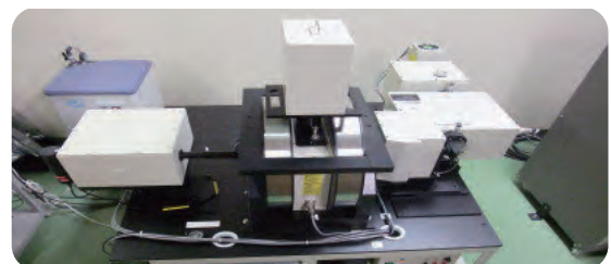
分光式磁気光学効果測定装置 (Spectroscopic Magneto-Optical Measurement System)
